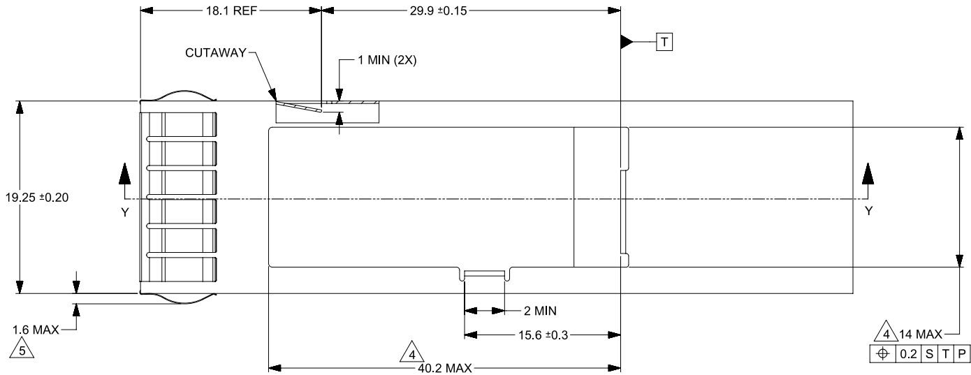
Figure 89: QSFP112 SMT 1x1 cage overview
