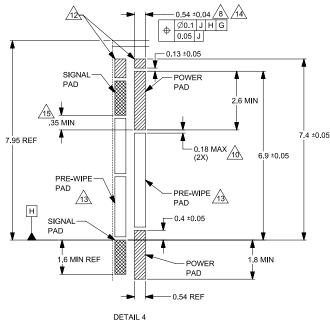
Figure 56: Detail module pad dimensions
