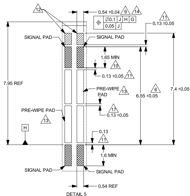
Figure 56: Detail module pad dimensions
