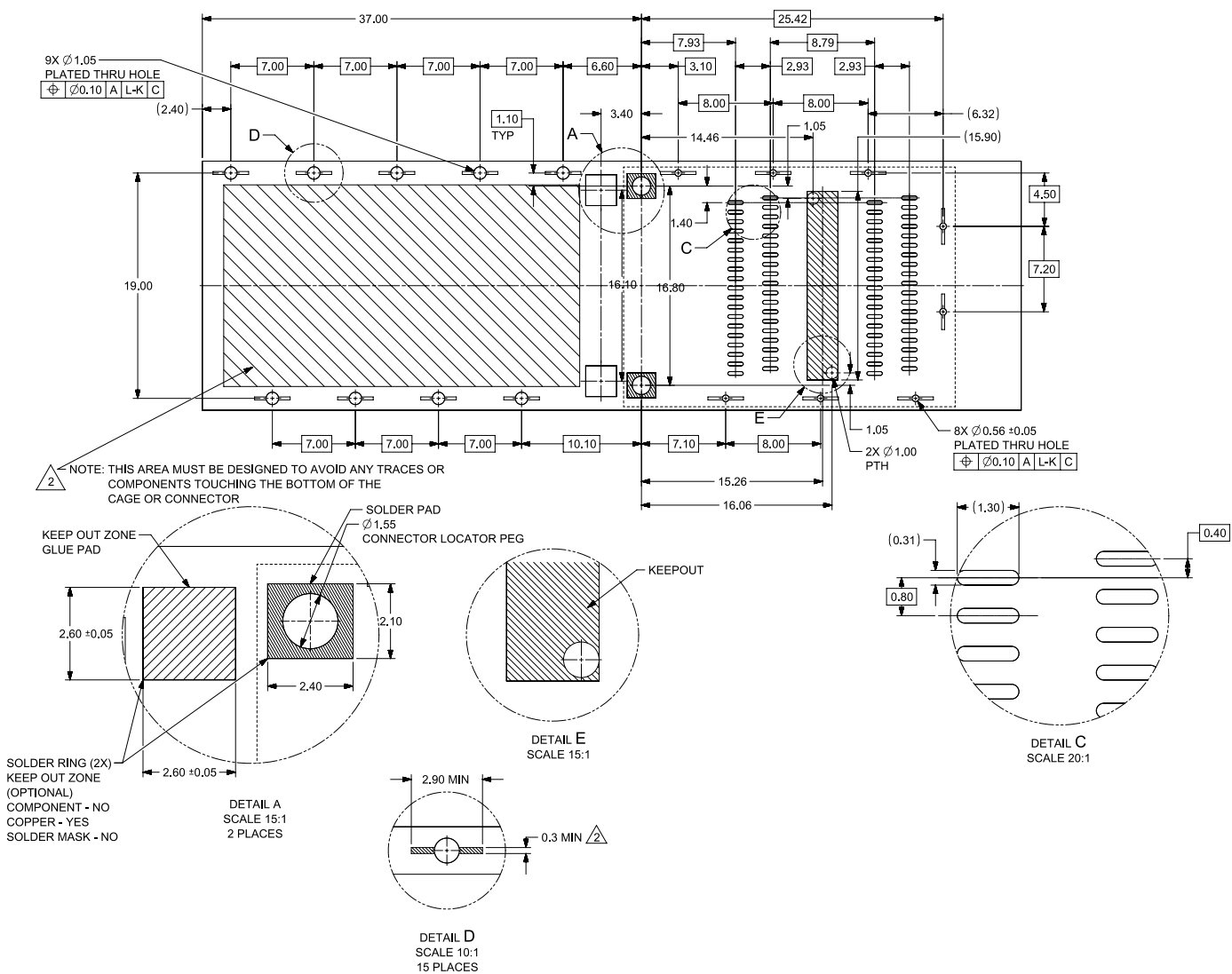
Figure 101: QSFP112 2x1 SMT connector host layout implementation 2
