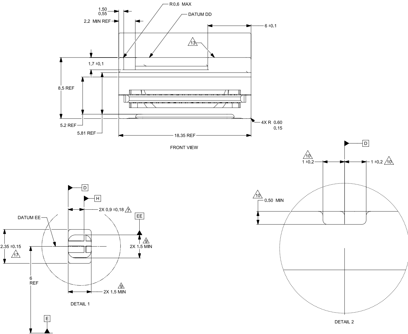
Figure 74: QSFP-DD800 module leading edge dimensions
