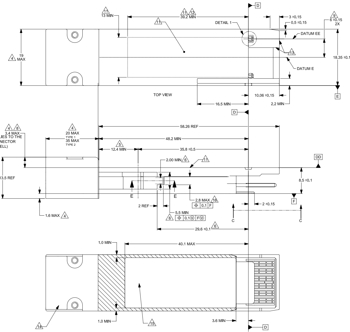
Figure 52: Drawing of the QSFP-DD module
