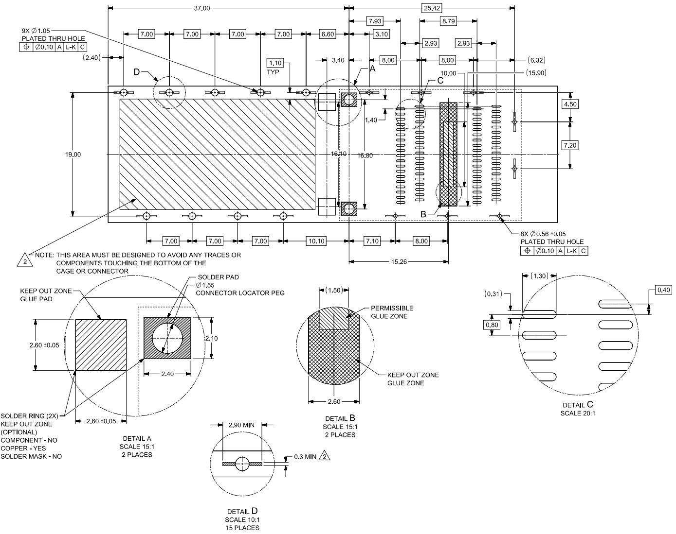
Figure 100: QSFP112 2x1 SMT connector host layout implementation 1
