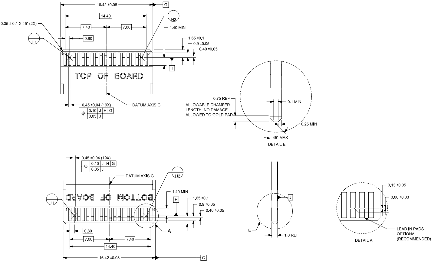
Figure 88 shows QSFP112 module paddle card dimensions. The QSFP112 connector can be integrated into a 1x1 or 2x1 stacked configuration with 1 or 2 ports as illustrated by Figure 90 and Figure 94.
