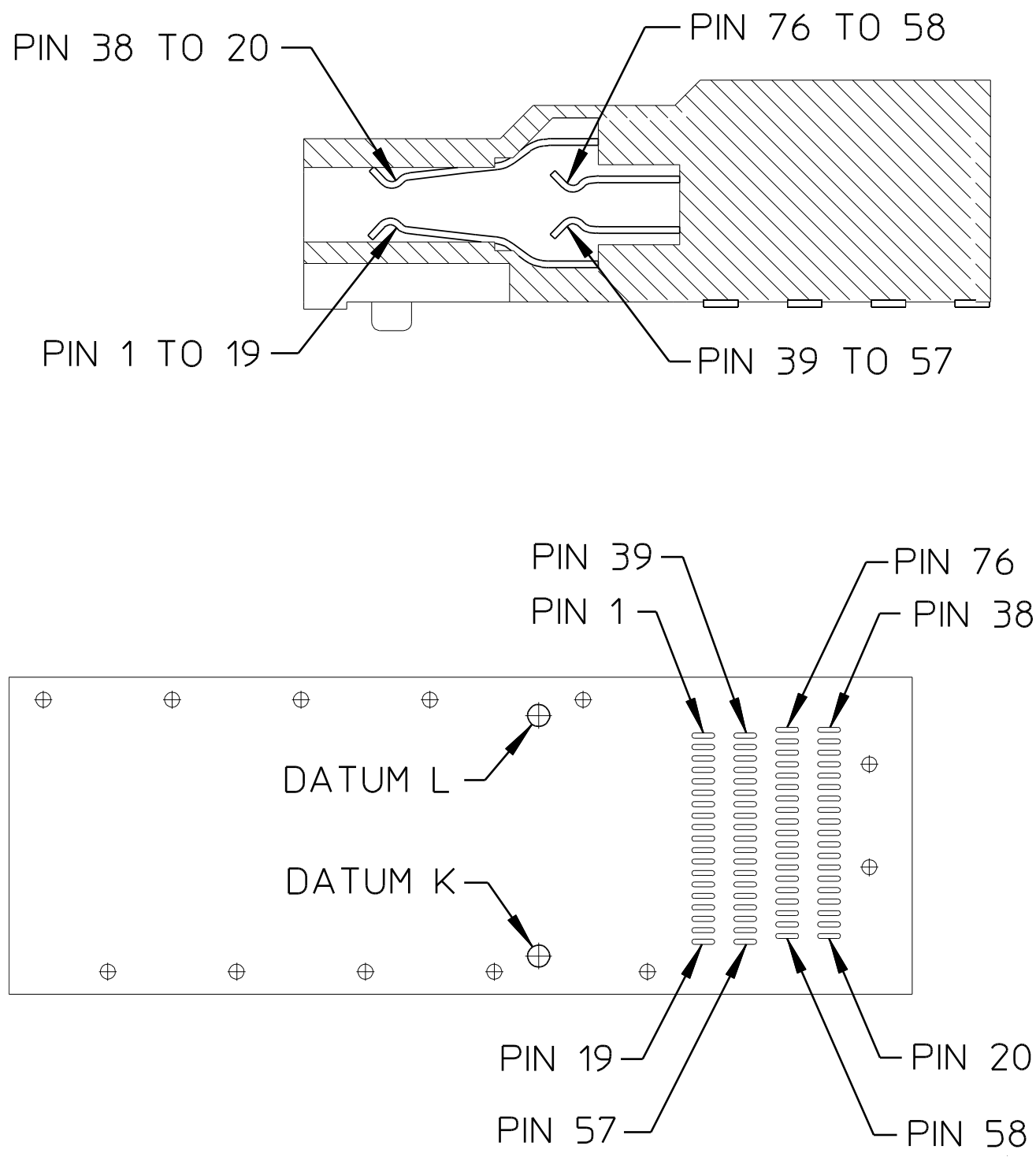
Figure 72: SMT Connector and host PCB contact numbers
