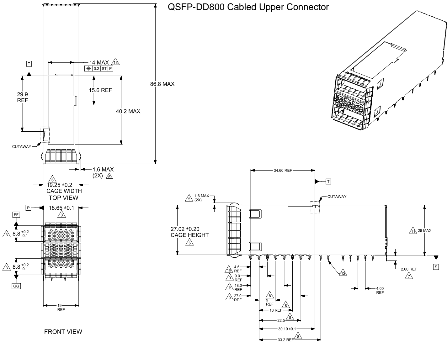
Figure 118: 2x1 Cabled over SMT connector and cage - Top View
