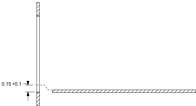
SECTION A-A Figure 82: 2x1 SMT Bezel Opening
