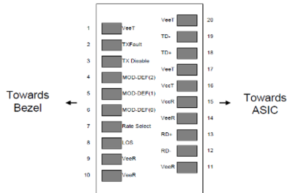
Figure 2: Pin-out of Connector Block on Host Board
